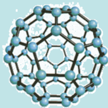
C_{60}
